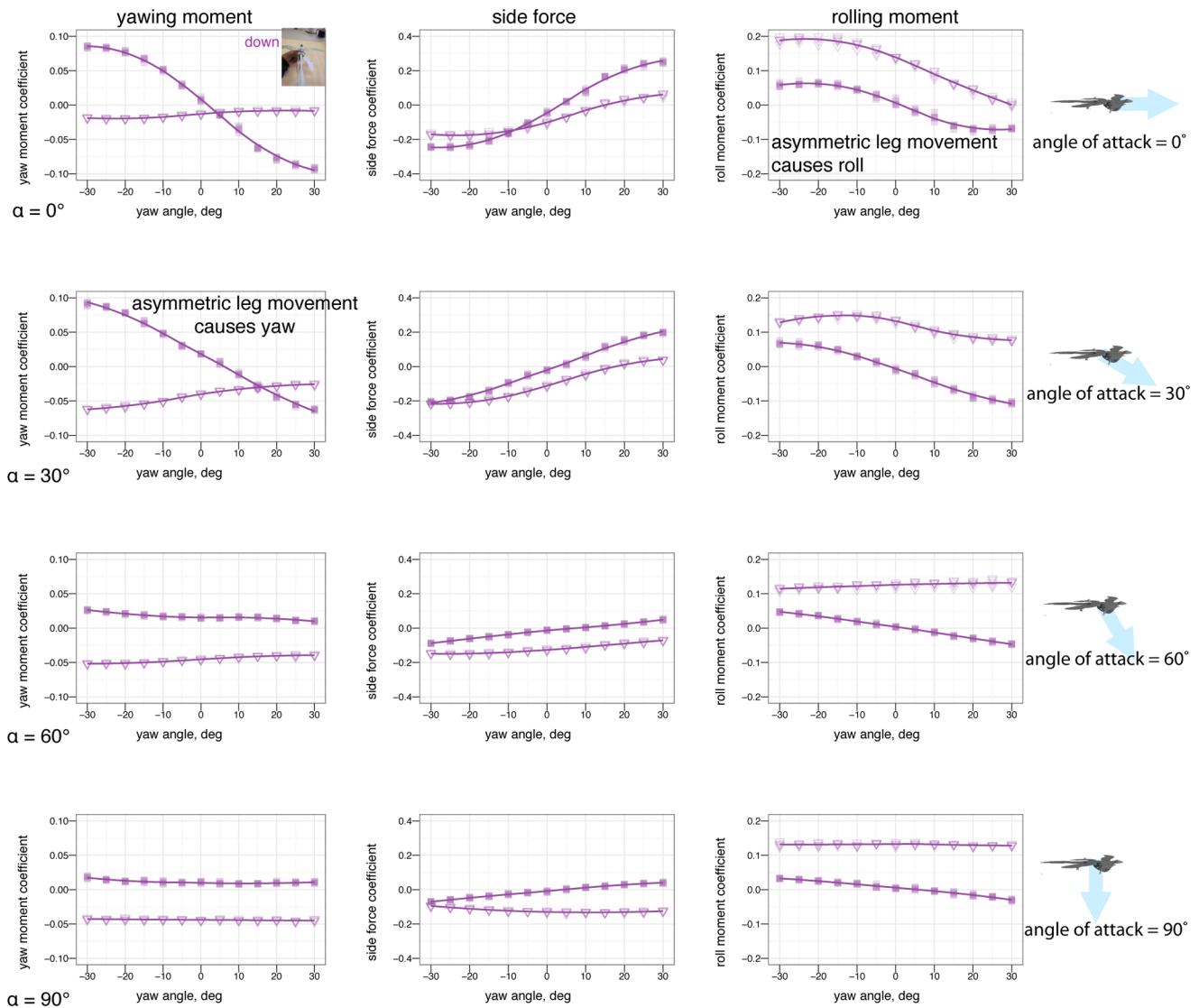
Figure 21. Asymmetric leg dihedral (leg dégagé , see inset) effect on yaw. Baseline down position (solid square) versus one leg at 45^\circ dihedral (down arrow). Placing one leg at a dihedral is destabilizing in yaw and produces side force and rolling and yawing moments due to the asymmetry. doi:10.1371/journal.pone.0085203.g021
