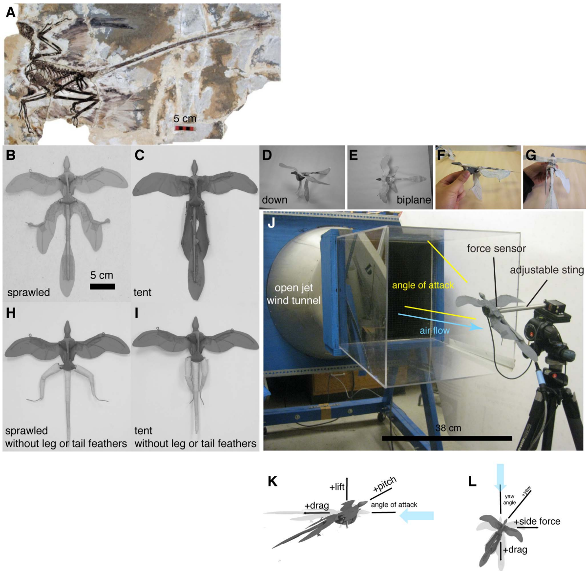
Figure 1. † Microraptor gui from [2], a dromaeosaur from the Cretaceous Jiufotang Formation of Liaoning, China; physical models, and sign conventions. A, Holotype specimen IVPP V13352, scale bar 5 cm. Notable features include semilunate carpal bones, a boomerang-shaped furcula, a shield-shaped sternum without a keel, uncinata processes on the ribs, unfused digits, an intermediate angle of the scapulocoracoid, and a long tail of roughly snout-vent length. In addition, there are impressions of feathers on the forelimbs, hindlimbs, and tail. B–J, Physical models of † M. gui , scale model wingspan 20 cm, snout-vent-length 8 cm. Reconstruction postures, B–I, used for constructing physical models: B, sprawled, after [2]; C, tent, after [34,58]; D, legs-down, after [34]; E, biplane, after [32]. F–I additional manipulations: F, asymmetric leg posture with 9090° leg mismatch (arabesque); G, example asymmetric leg posture with 45° dihedral on one leg (dégagé); H, sprawled without leg or tail feathers; I, tent without leg or tail feathers. J, test setup; K, sign conventions, rotation angles, and definitions for model testing, after [10,30,31]. doi:10.1371/journal.pone.0085203.g001
